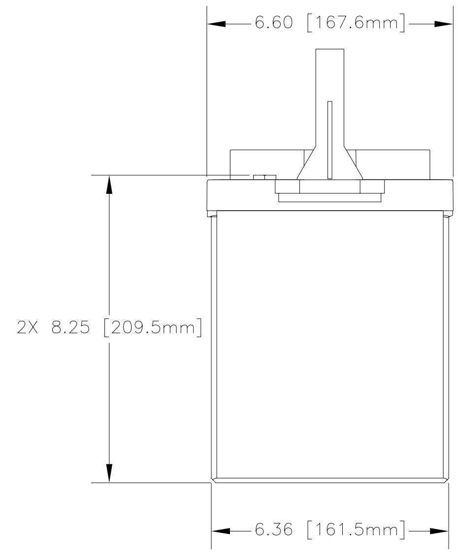
ENVELOPE DRAWING
