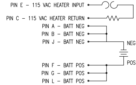
CONNECTOR SCHEMATIC DIAGRAM
