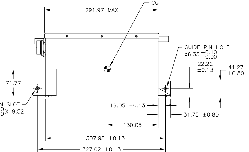
ENVELOPE DRAWING
