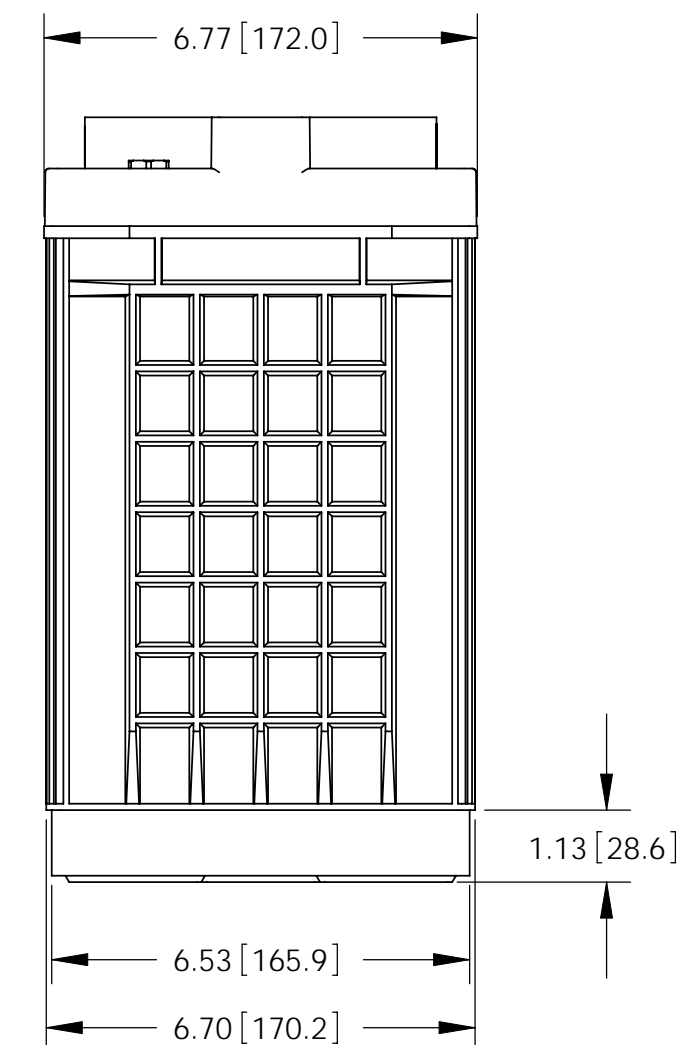
ENVELOPE DRAWING
