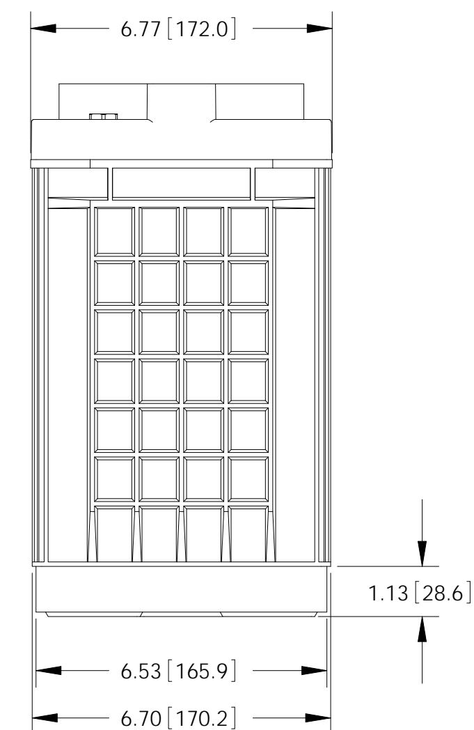
ENVELOPE DRAWING
